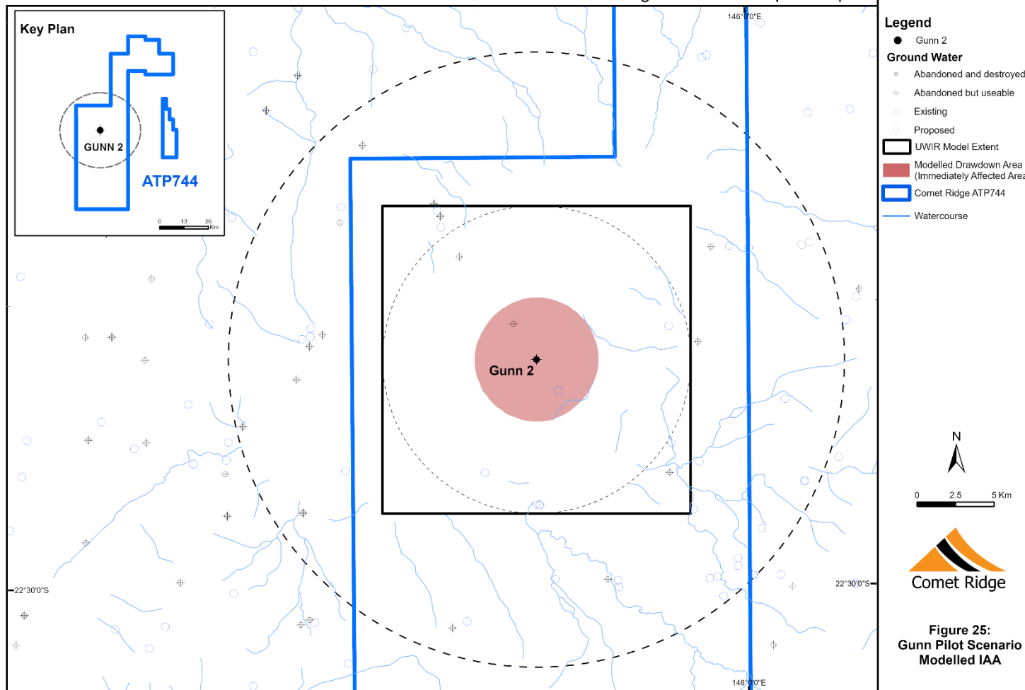
Figure 25: Modelled IAA: proposed five well vertical pilot scenario
