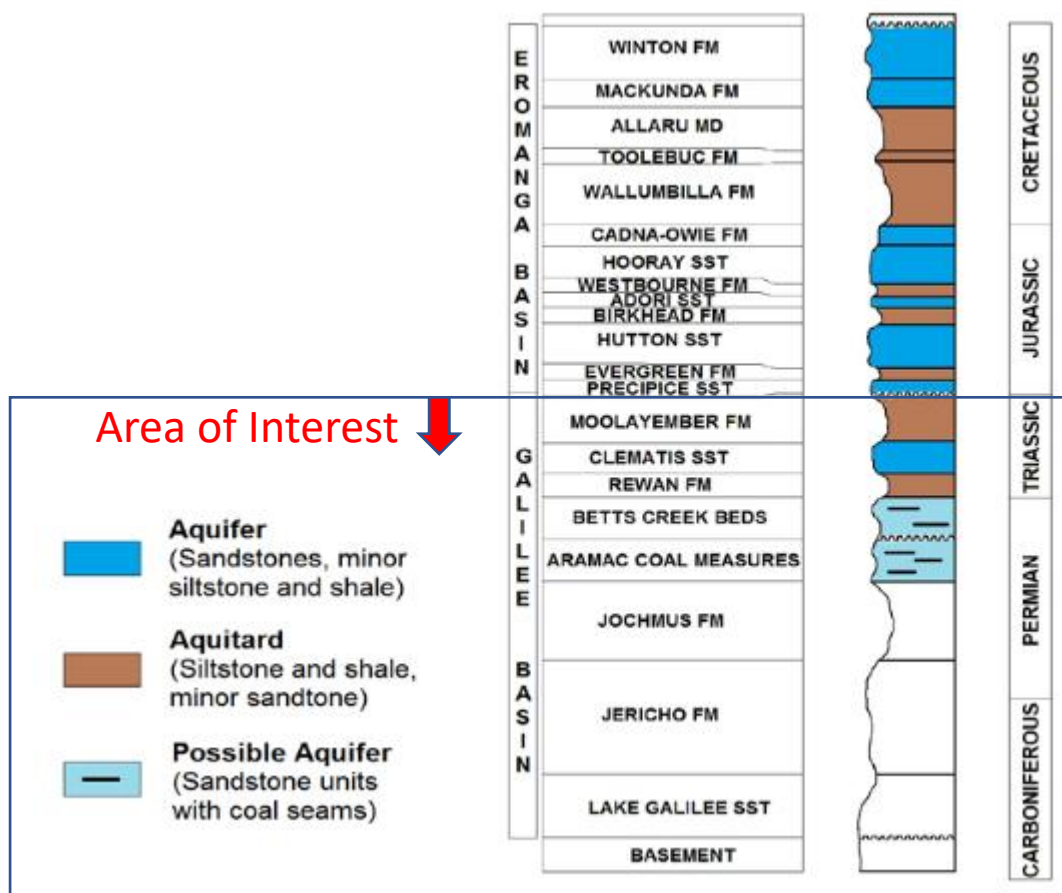
Figure 39: Simplified hydrostratigraphy in the Galilee and Eromanga Basins (after Mooya, 2011)
