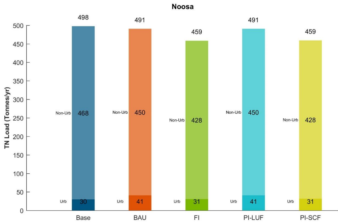
Figure 3-104 TN catchment loads from Noosa
