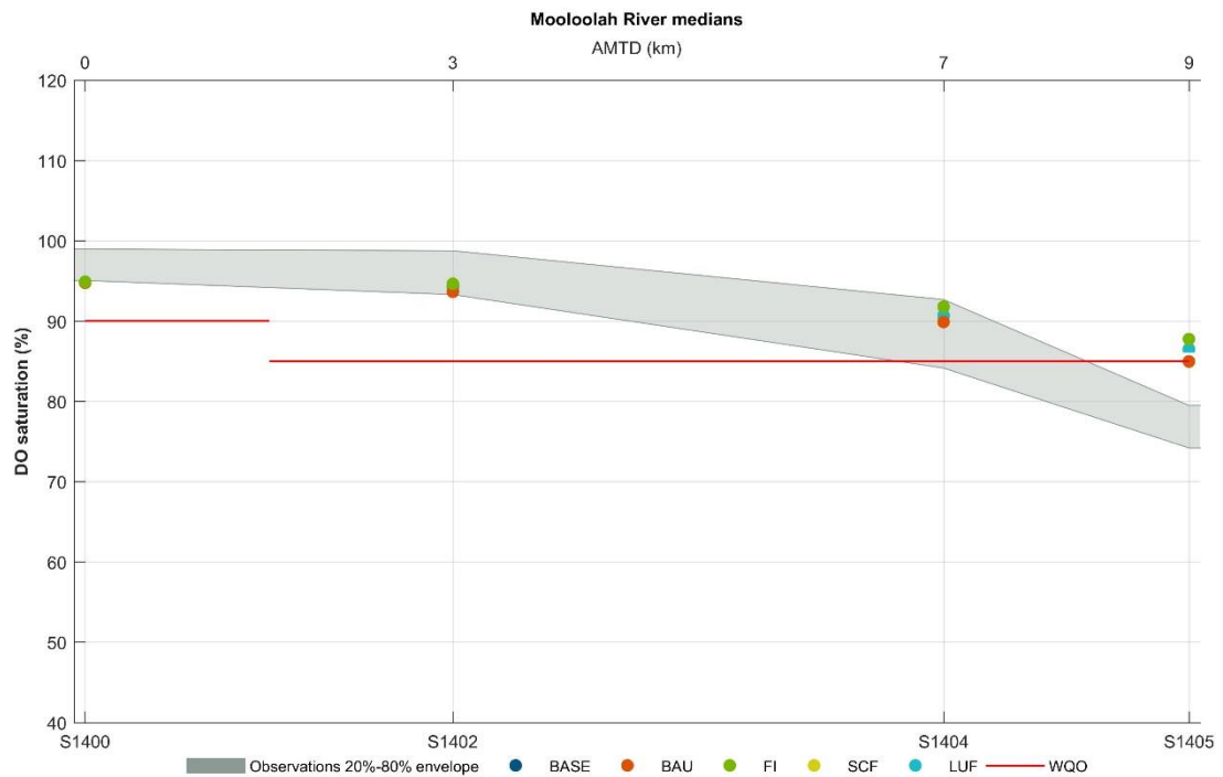
Figure 3-15 Comparison of DO saturation medians across scenarios for Mooloolah
