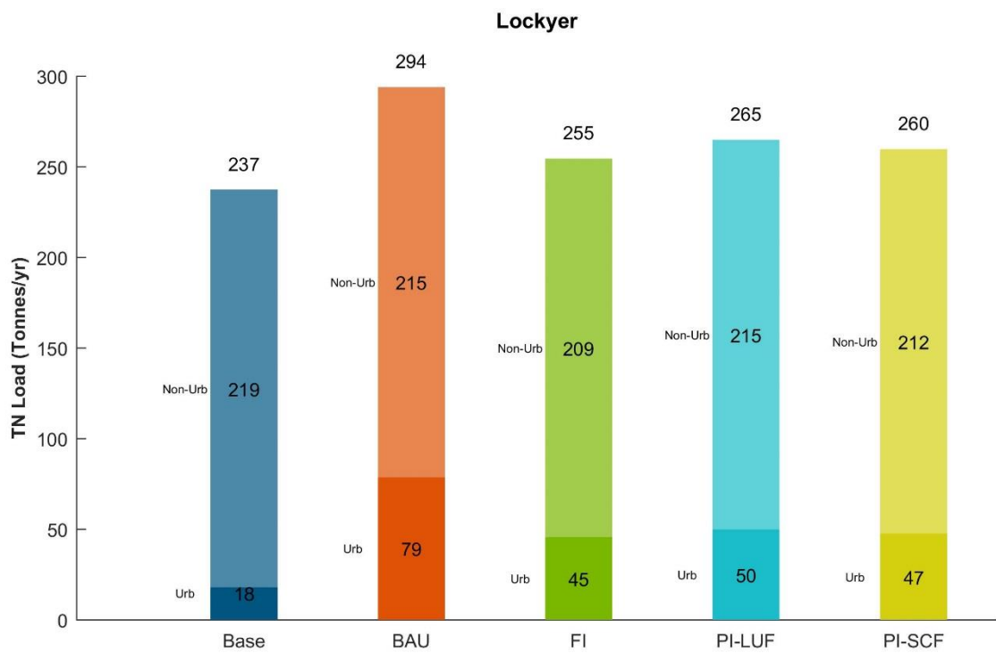
Figure 3-54 TN catchment loads from Lockyer
