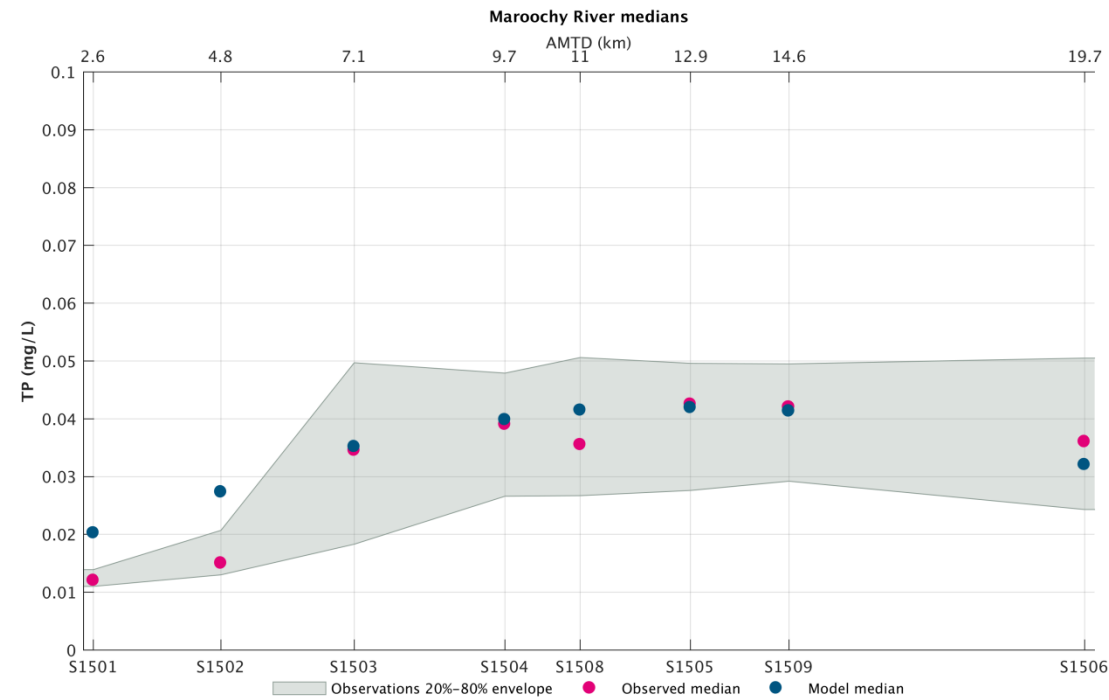
Figure A-15 Total phosphorus thalweg comparison
