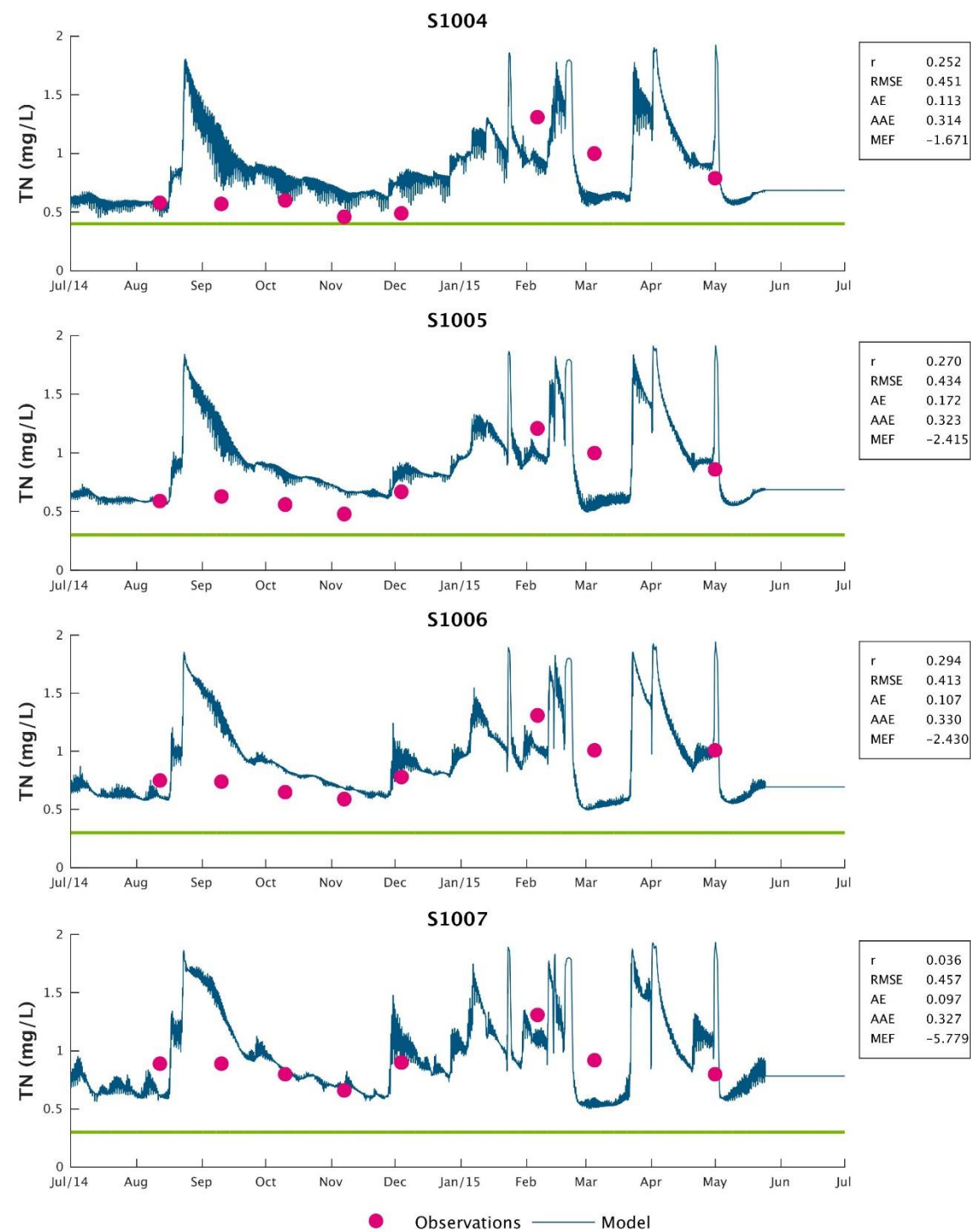
Figure A-56 Total Nitrogen timeseries plot for Caboolture U/s
