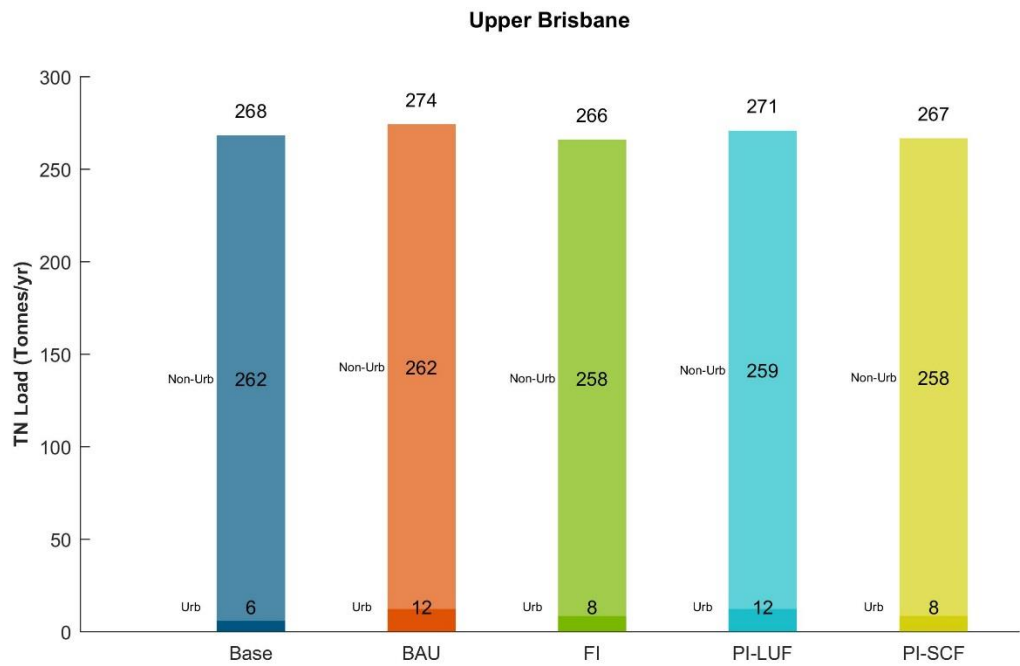
Figure 3-45 TN catchment loads from Upper Brisbane
