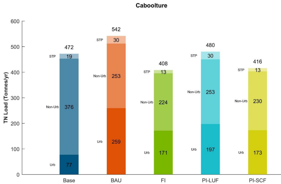
Figure 3-29 TN catchment loads from Caboolture
