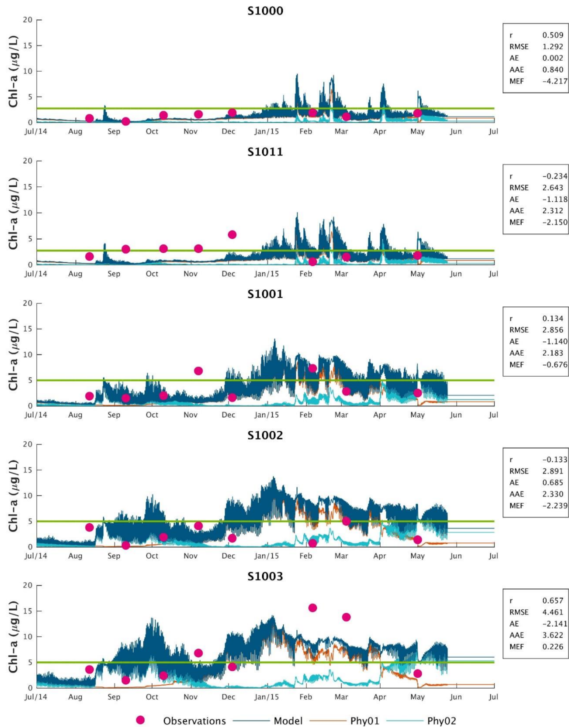
Figure A-61 Chlorophyll-a timeseries plot for Cabooture D/s
