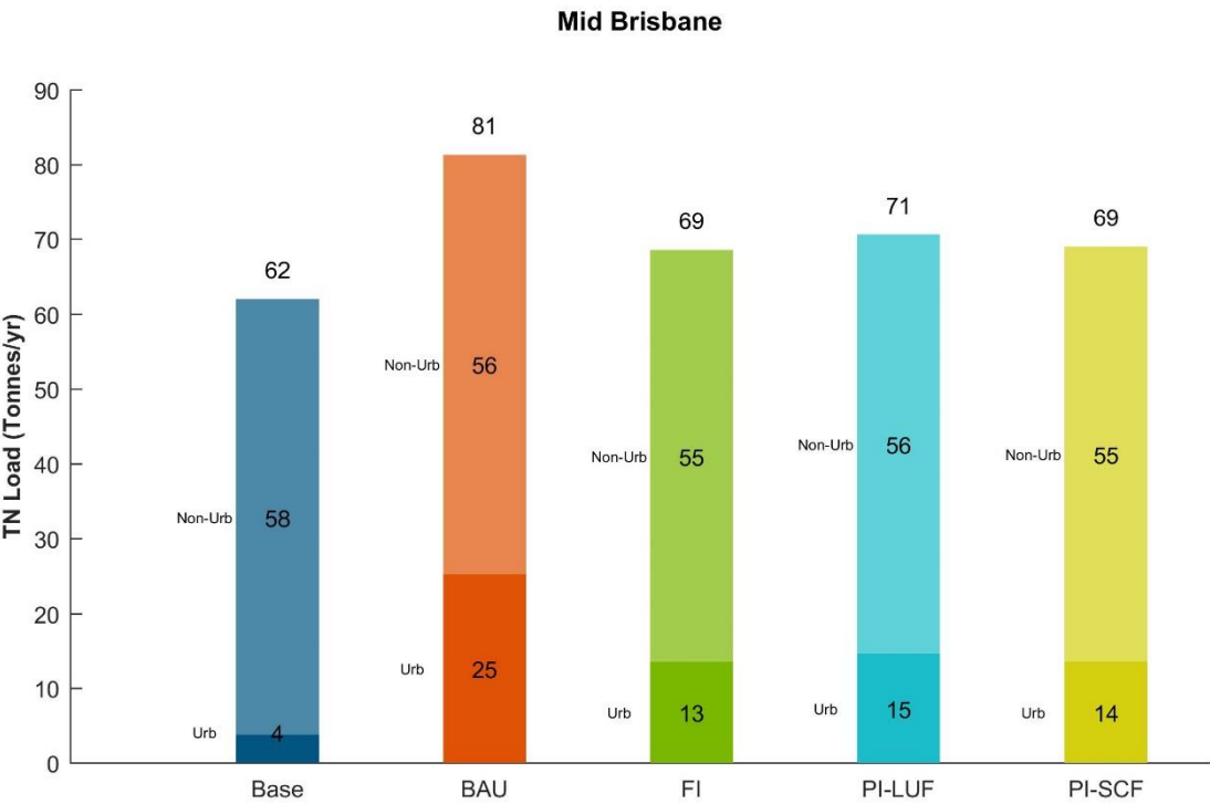
Figure 3-51 TN catchment loads from Mid Brisbane
