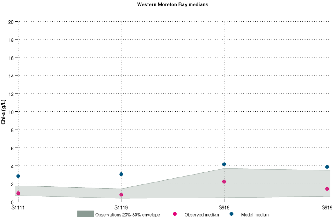
Figure A-158 Chlorophyll-a thalweg comparison Moreton Bay - Western
