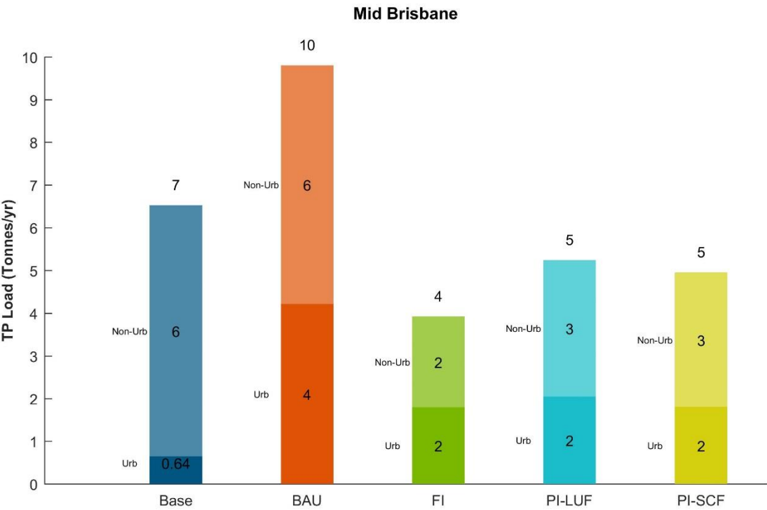
Figure 3-52 TP catchment loads from Mid Brisbane
