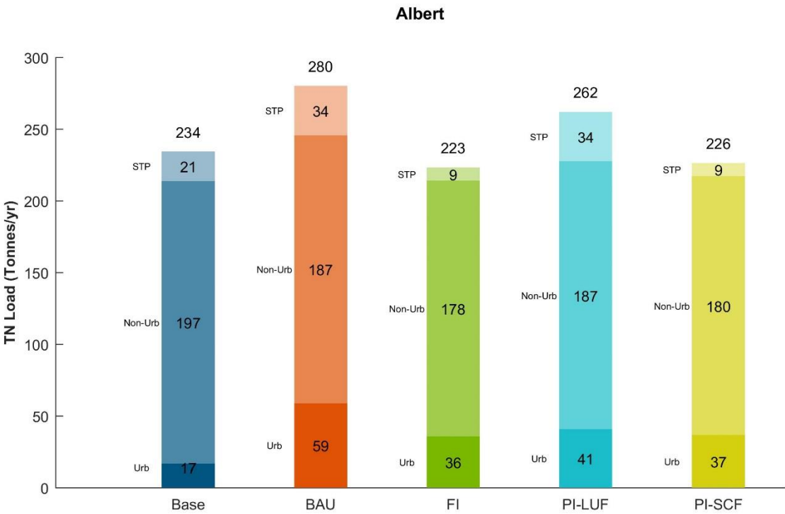
Figure 3-76 TN catchment loads from Albert
