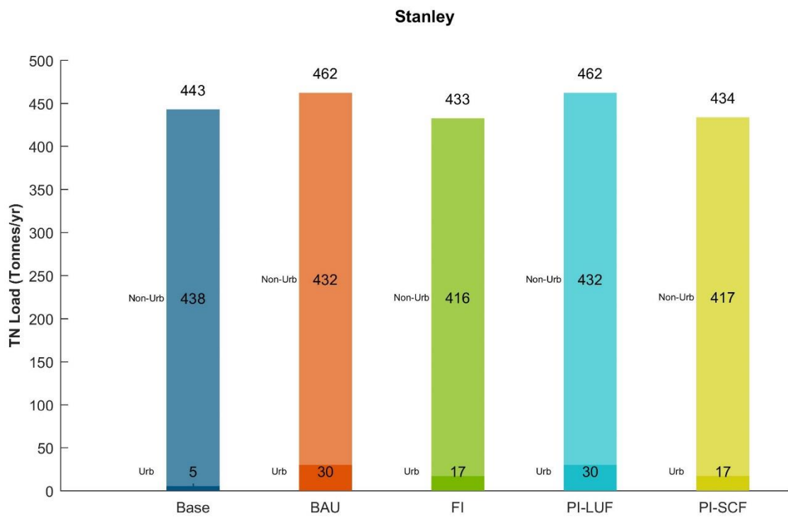
Figure 3-48 TN catchment loads from Stanley
