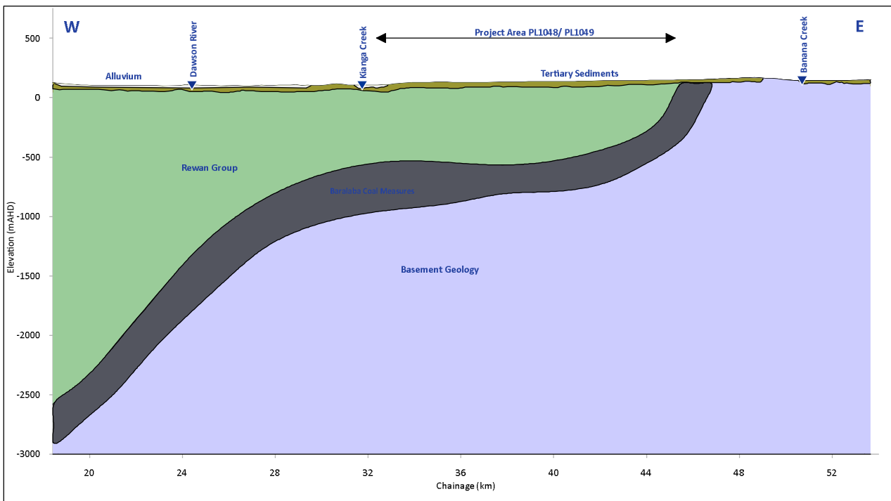
Figure 5-3 West – East Conceptual Geological Cross-section across the Project Area
