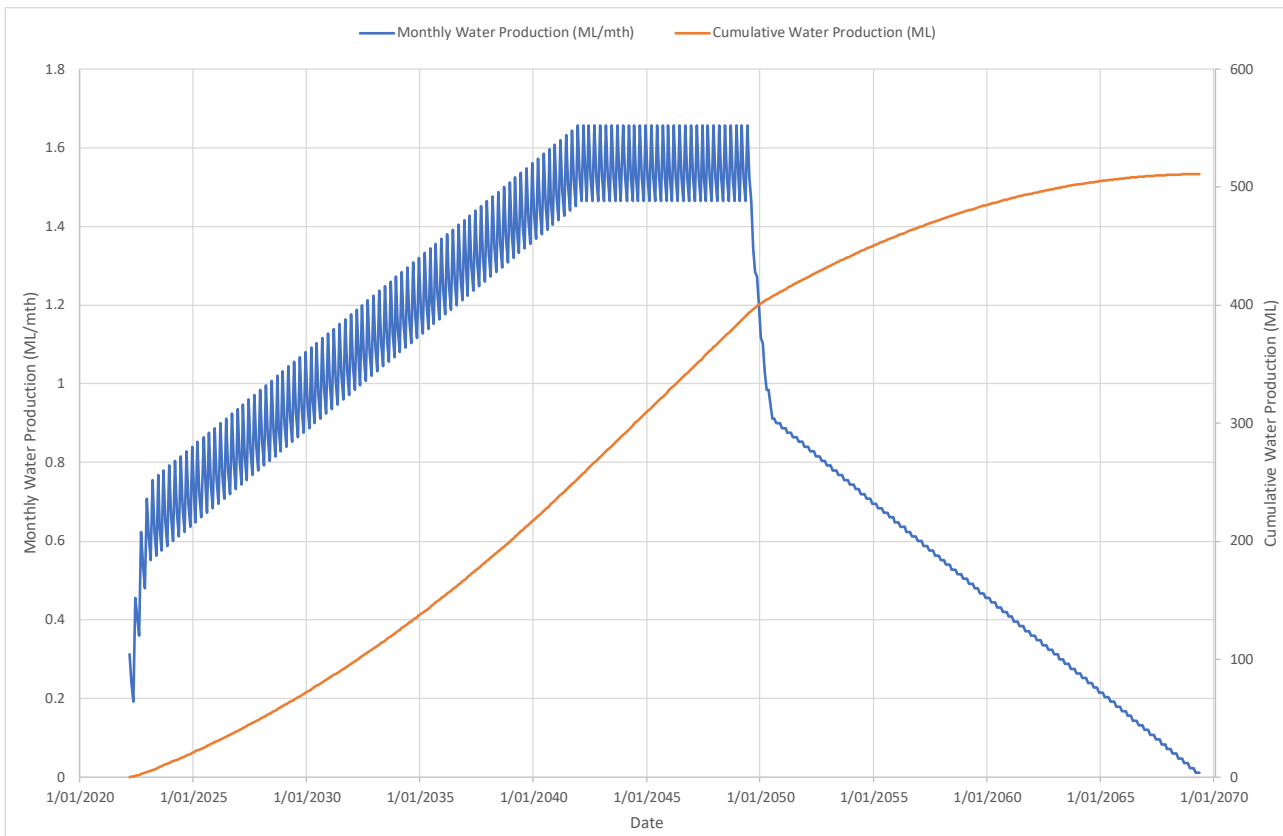
Figure 7-1 Predicted Water Production Rate and Cumulative Volume for the Project
