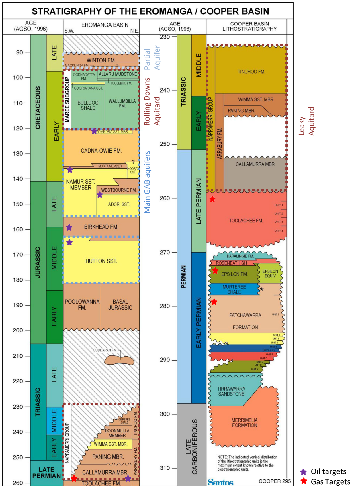
Figure 5.3 Regional Stratigraphy in the Cooper and Eromanga Basins
