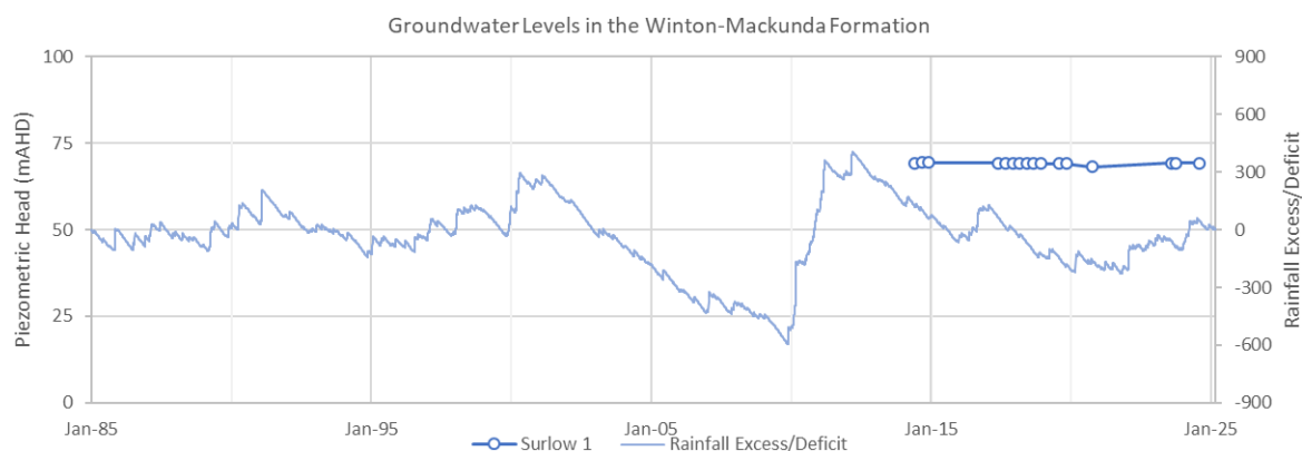
Figure 7.5 Groundwater Elevation Hydrograph – Winton-Mackunda Formation
