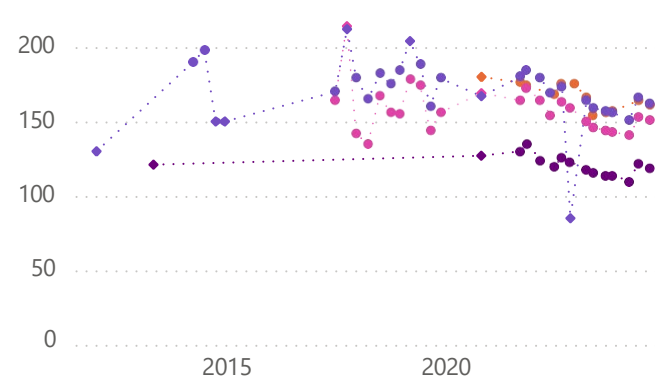
Chloride (mg/L)
