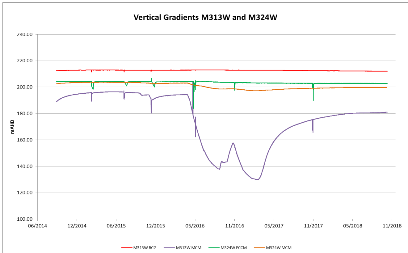
Figure 17: Site 2 - Review of Vertical Gradients for M313W and M324W
