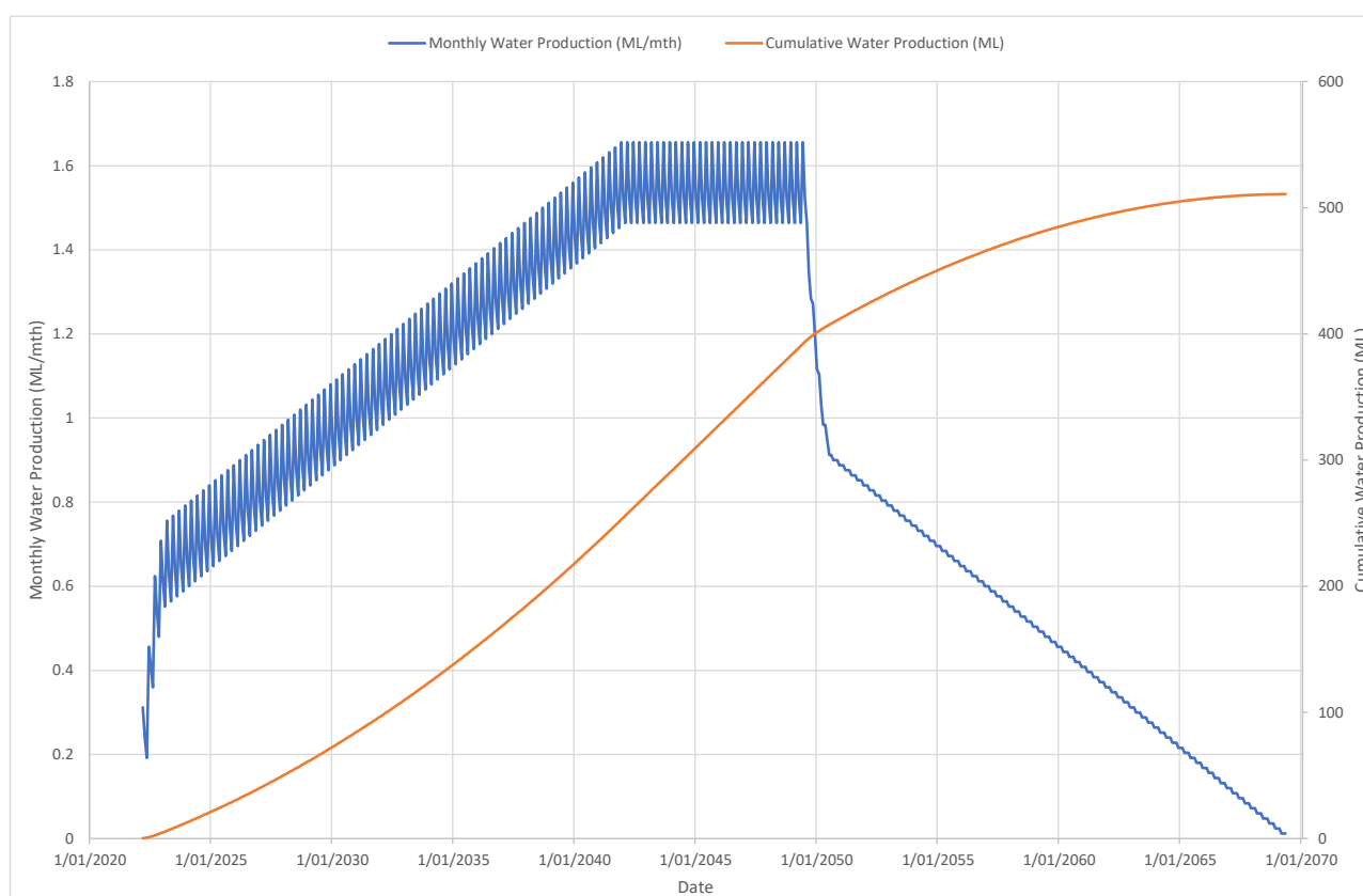
Figure 6.2 Predicted Water Production Rate and Cumulative Volume for the Project
