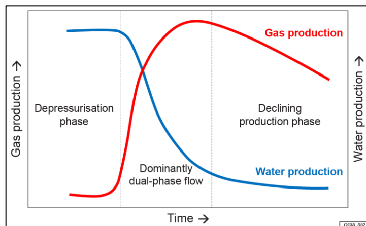
Figure 3-2: Typical gas and water flow profile during CSG production
