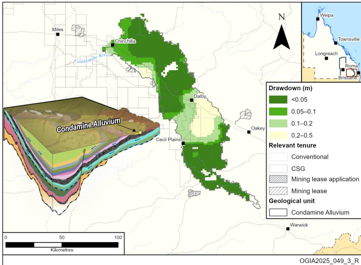
Figure 10-8: Long-term impact distribution, Condamine Alluvium
