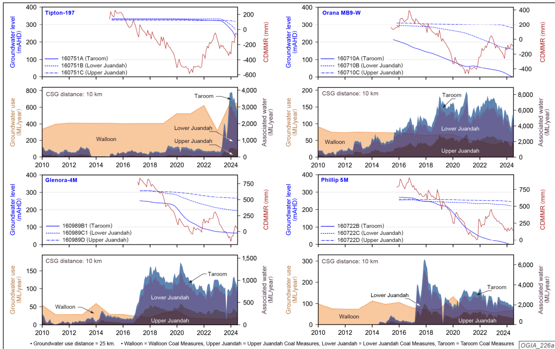
Figure 9-4: Groundwater level trends at selected sites in the Walloon Coal Measures
