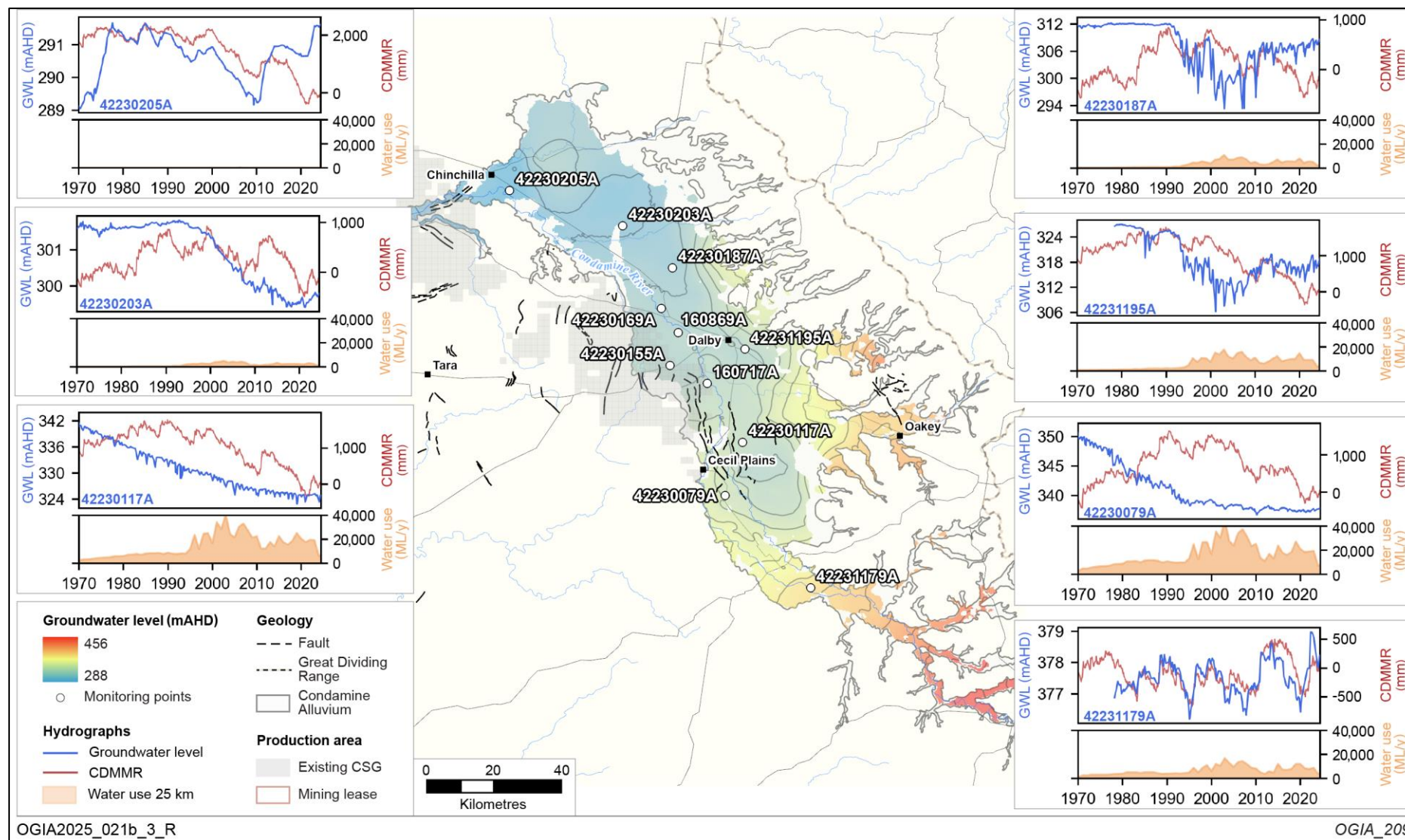
Figure 9-23: Example hydrographs showing trends and the potentiometric surface in the Condamine Alluvium
