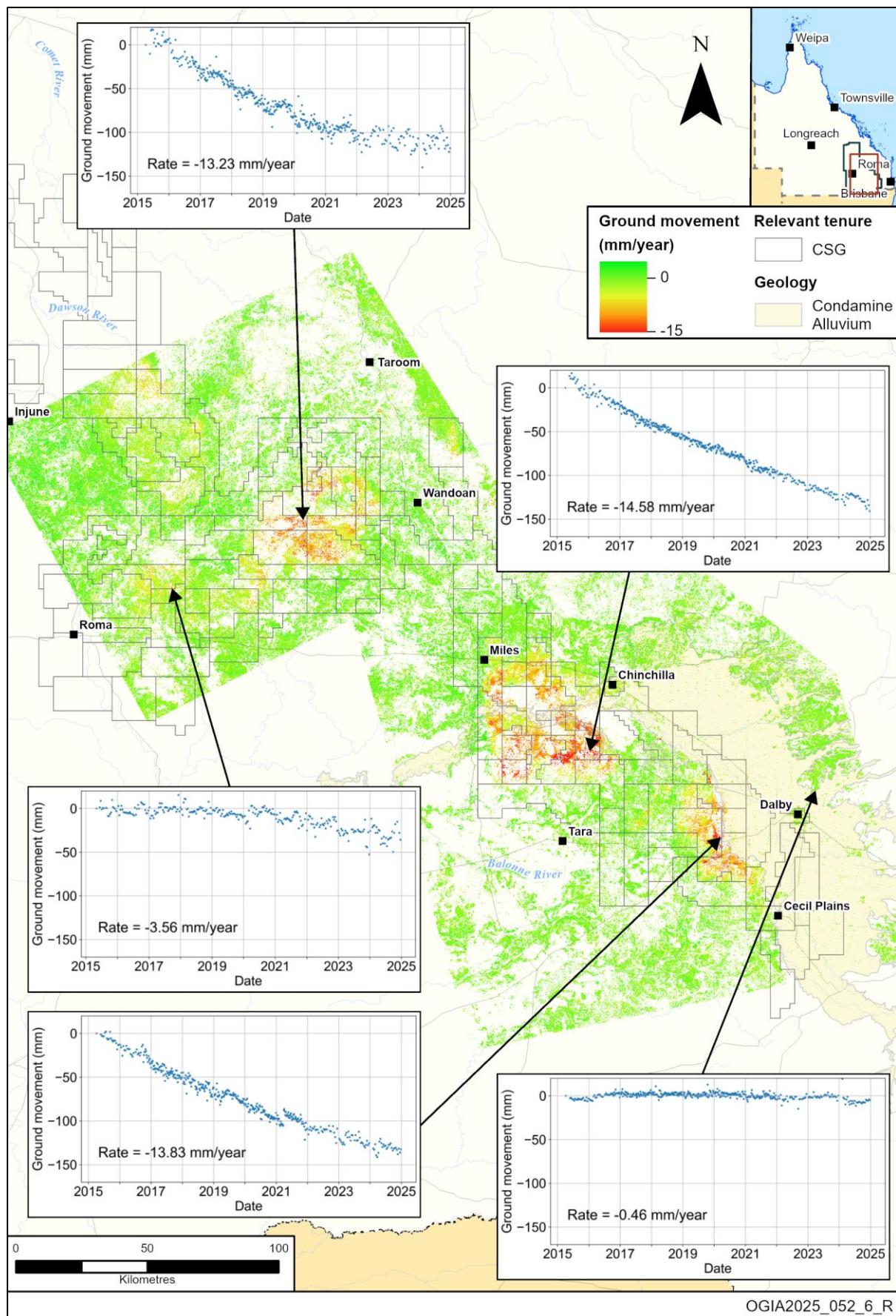
Figure 9-27: Spatial and temporal pattern of InSAR-derived ground motion around gas fields in the Surat CMA, 2015 to 2024 (Y. (Wendy) Zhang et al. 2025)
