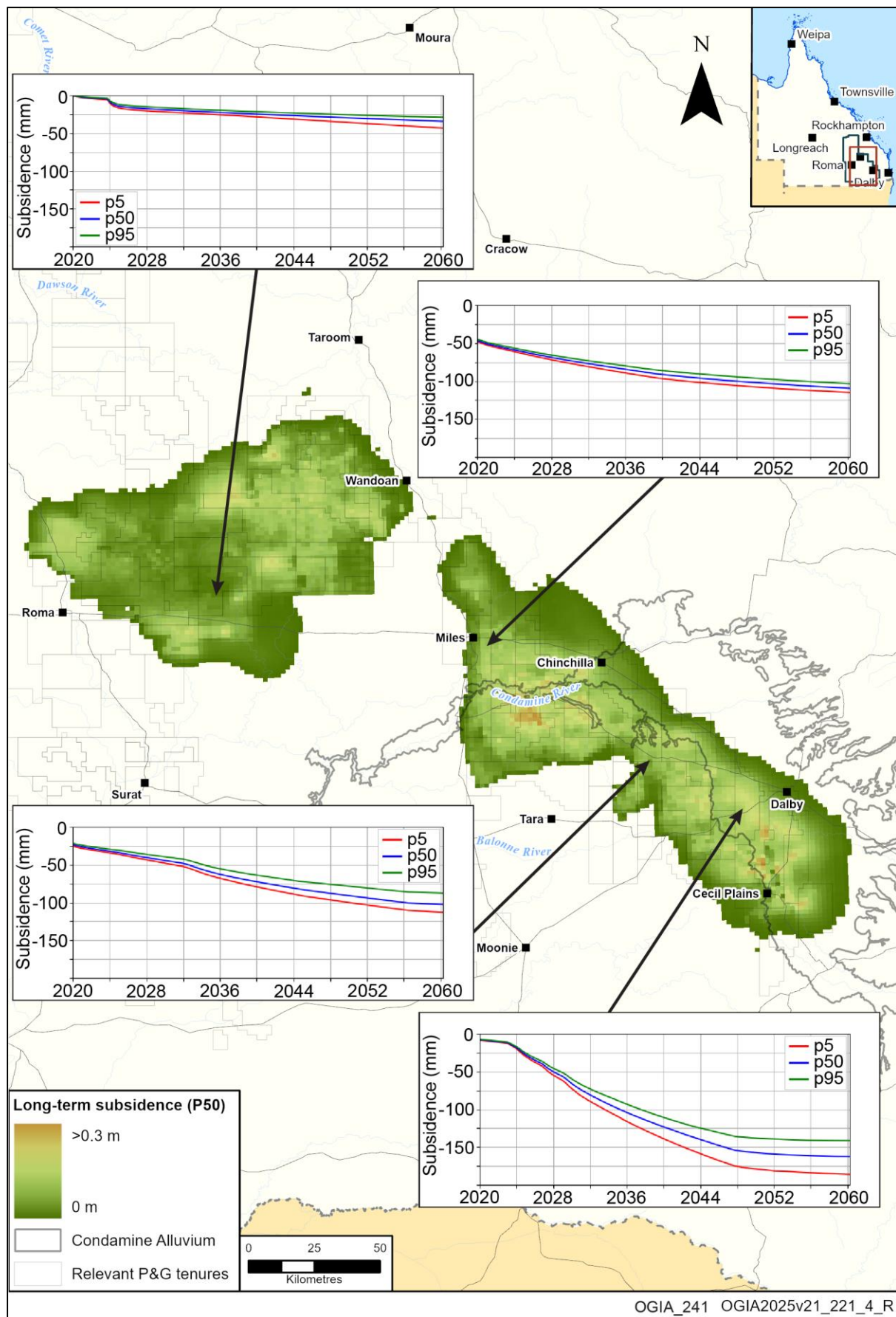
Figure 10-19: Predicted CSG-induced subsidence (P50) in the Surat Basin
