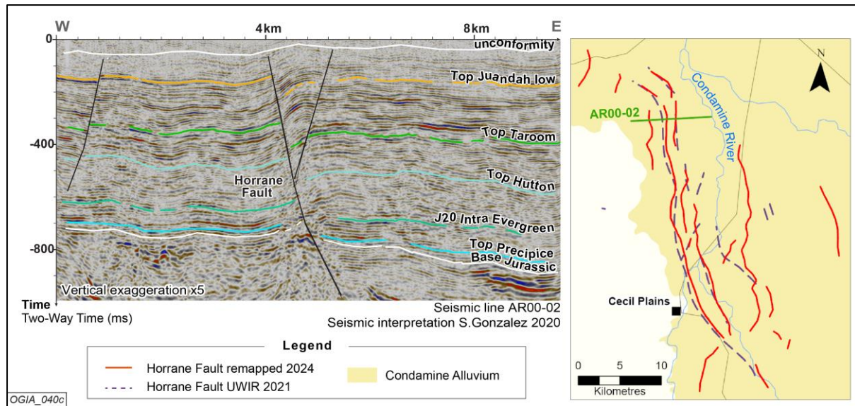
Figure 7-14: Horrane Fault revised mapping and interpretation
