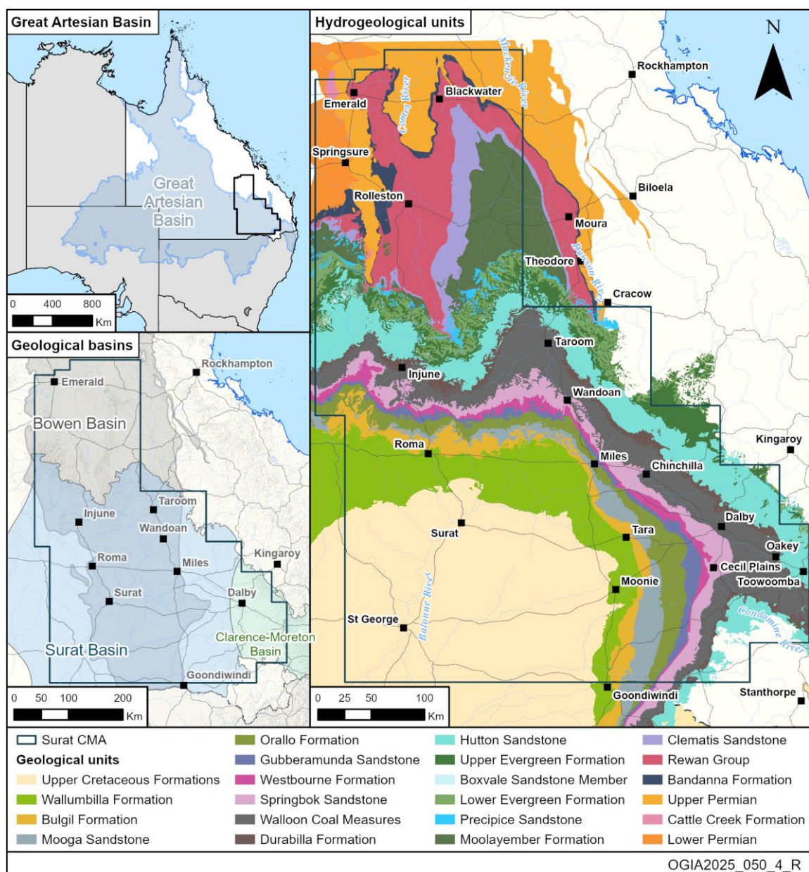
Figure 4-1: Great Artesian Basin (GAB), geological basins and subcropping hydrogeological units in relation to the Surat CMA
