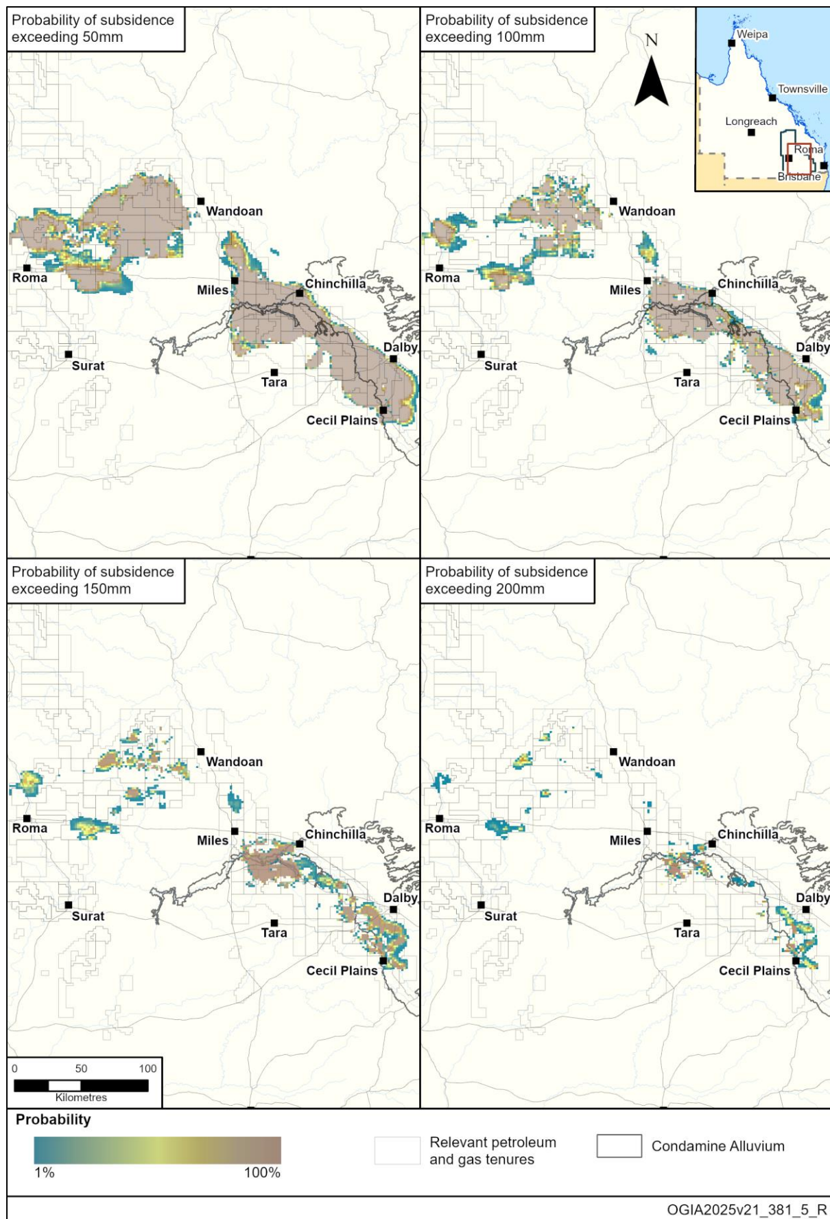
Figure 10-20: Probabilities of predicted subsidence across the Walloon Coal Measures footprint exceeding 50, 100, 150 and 200 mm by 2060
