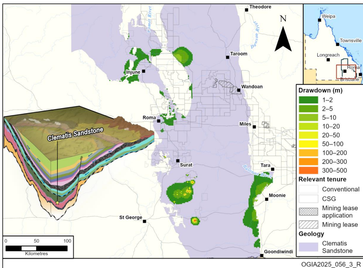
Figure 10-9: Long-term impact distribution, Clematis Sandstone
