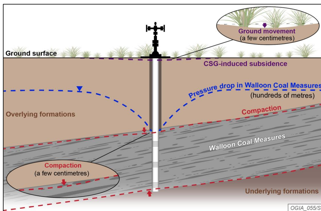
Figure 7-3: Schematic of the CSG-induced subsidence process
