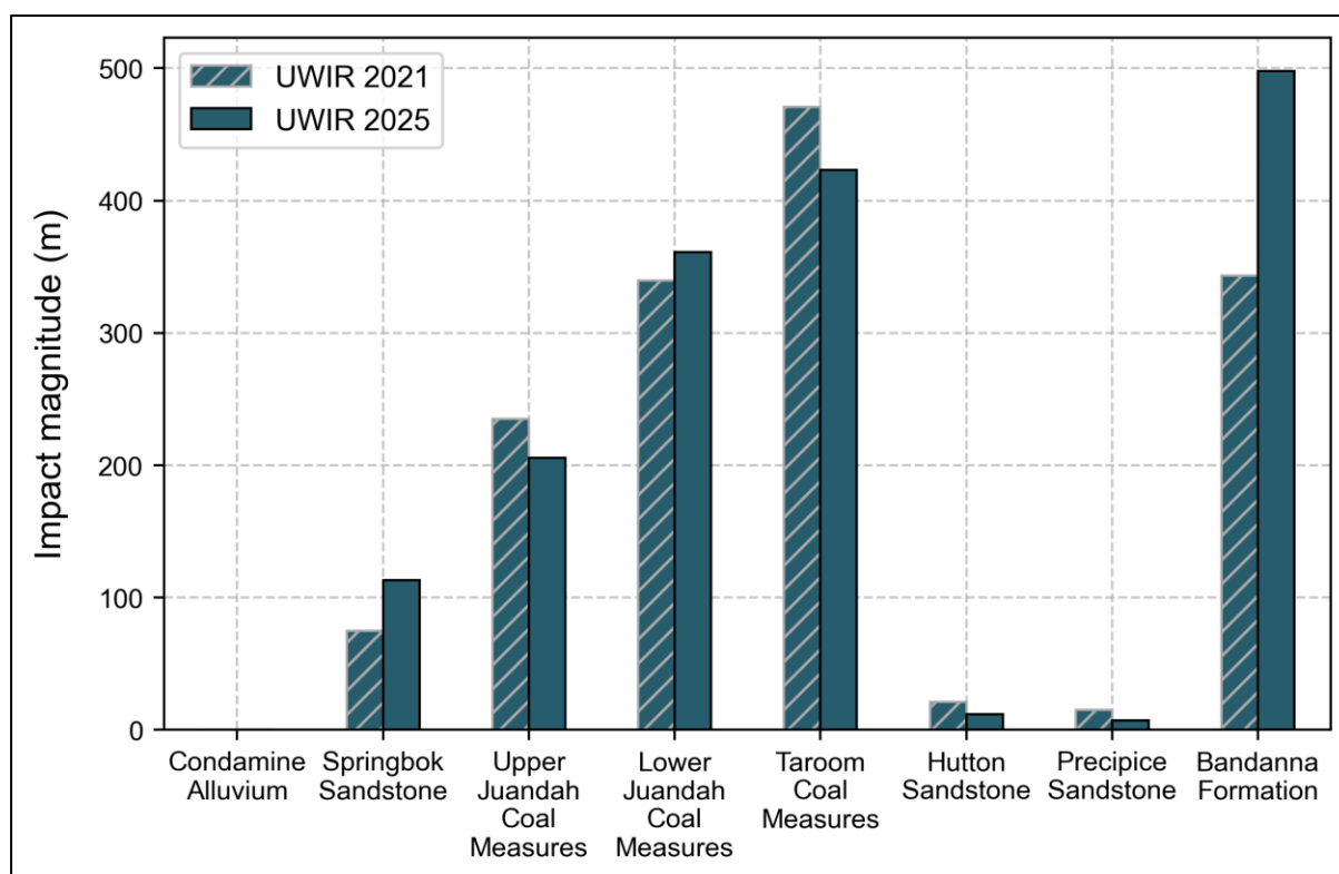
Figure 10-18: Comparison of P90 impact magnitude within the LAA
