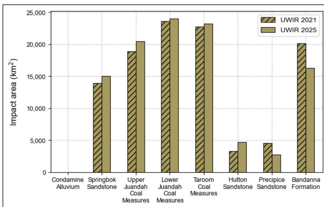
Figure 10-17: Comparison of impact area (LAA) for the relevant statutory trigger thresholds
