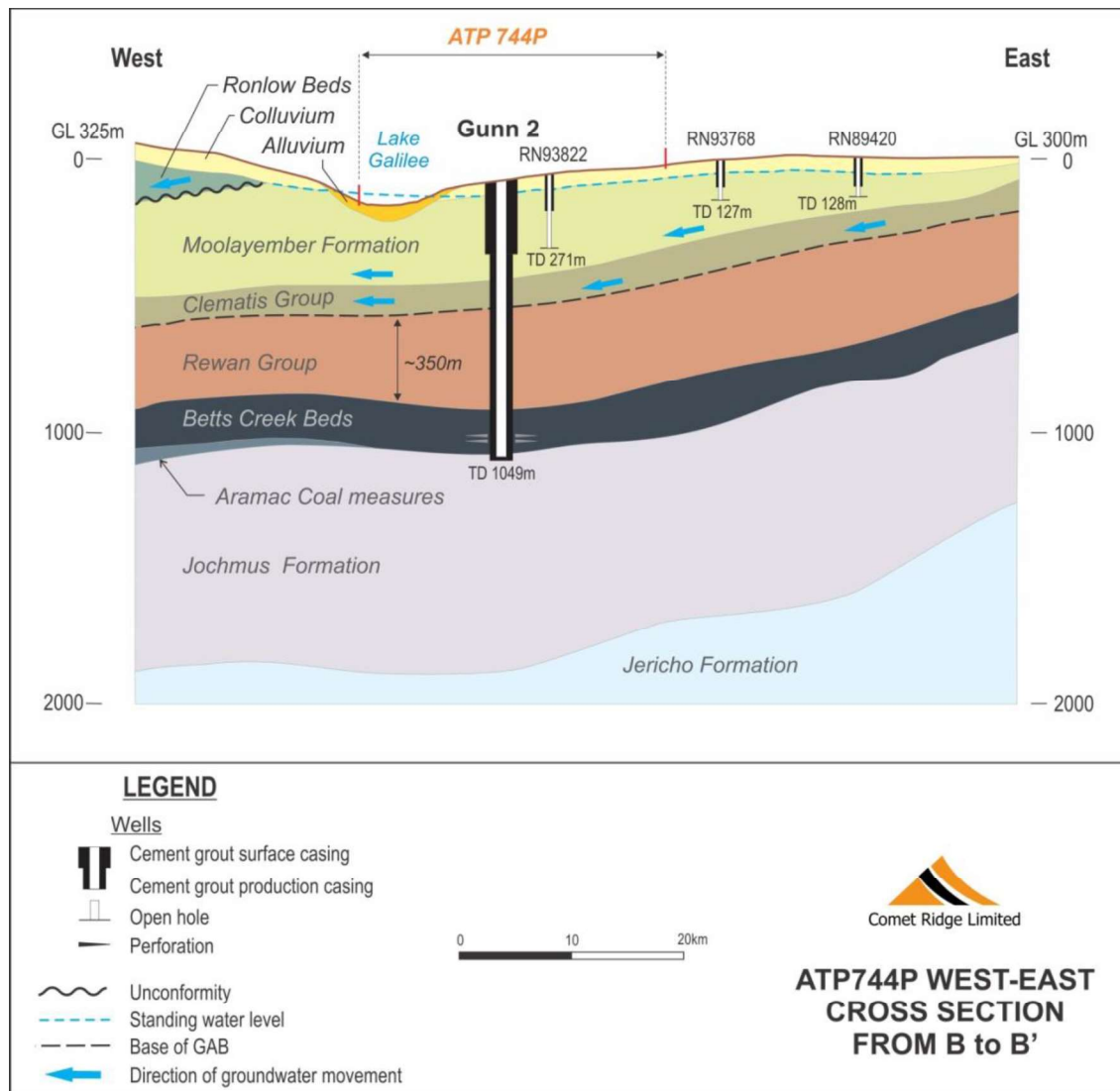
Figure 16: Schematic geological cross-section across ATP744, showing Gunn #2 appraisal well, nearby groundwater bores and groundwater flow direction.
