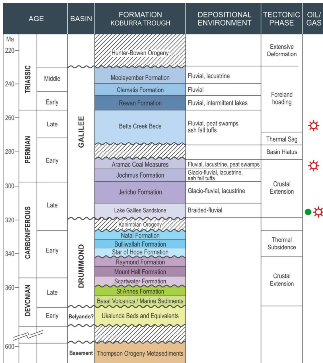
Figure 31. Regional Stratigraphy – Koburra Trough - Galilee Basin
