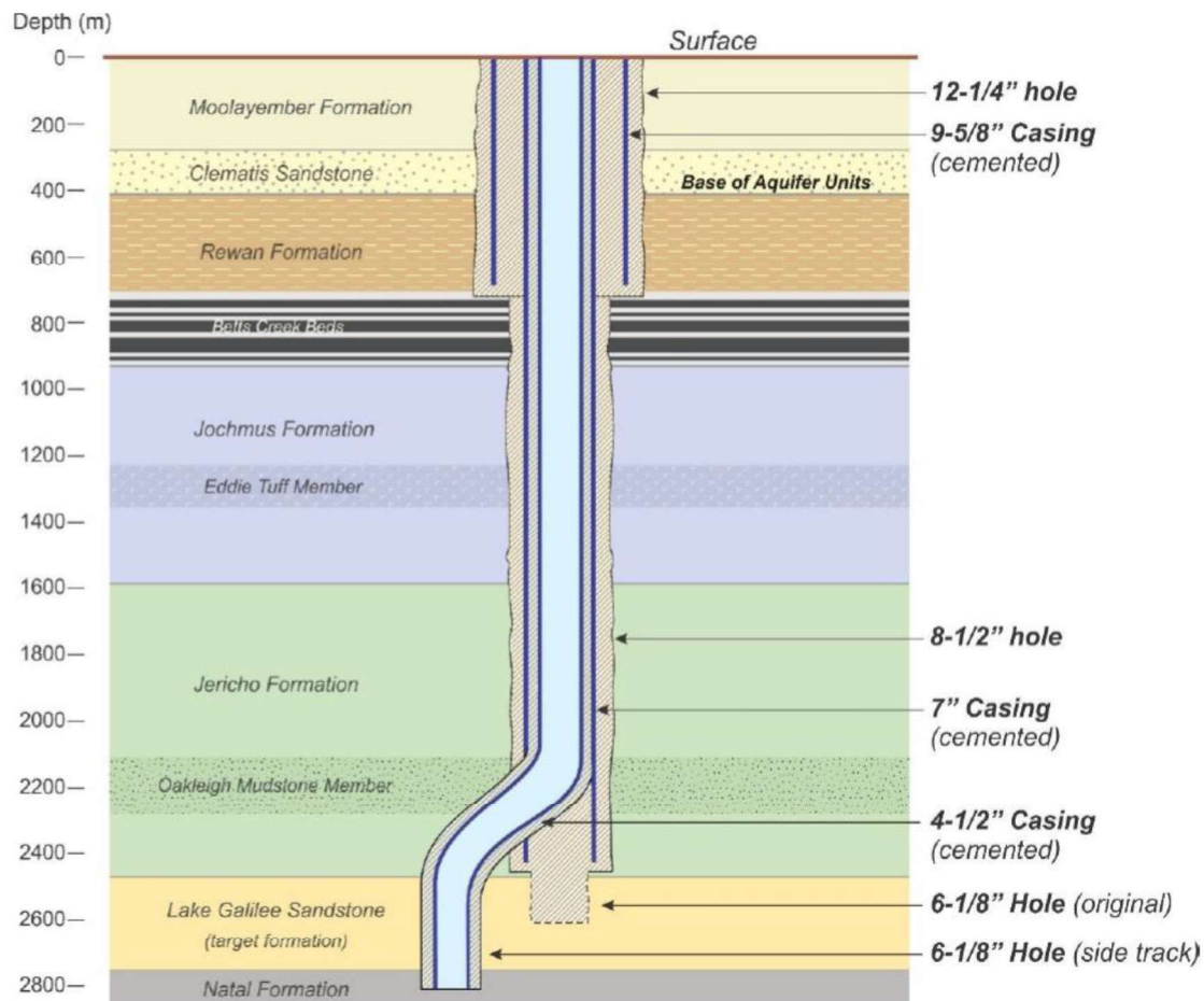
Figure 33. Albany 1 ST1 Well Design
