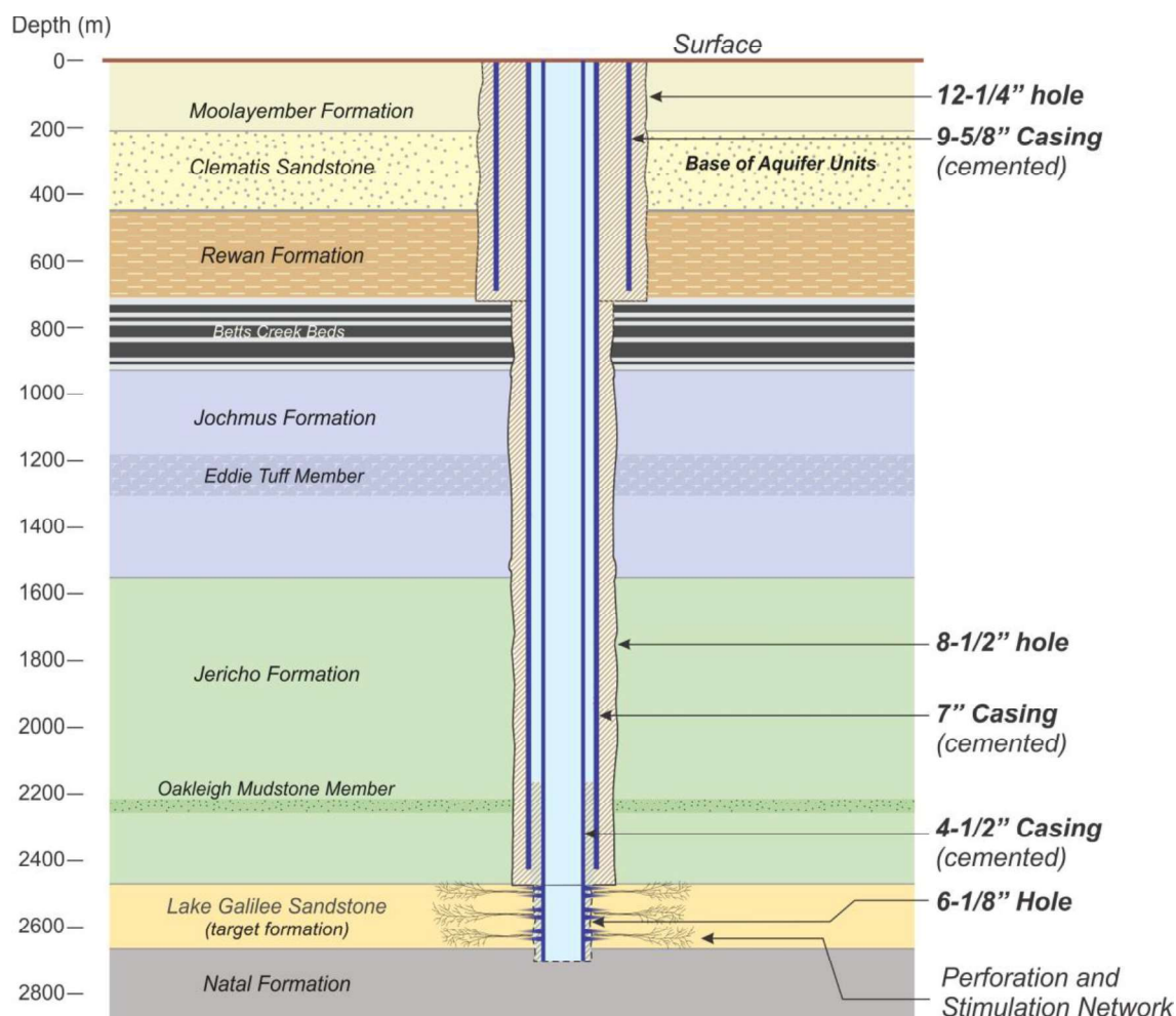
Figure 32. Albany 2 Well Design and Stimulation Schematic
