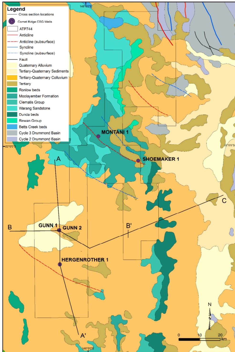
Figure 4: Surface geology map of ATP744, showing locations of schematic cross-sections.
