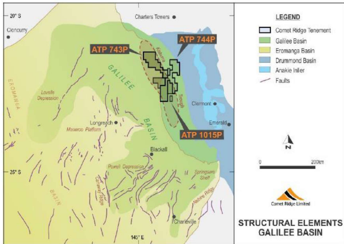
Figure 28. Comet Ridge Galilee Permits, showing regional structural elements
