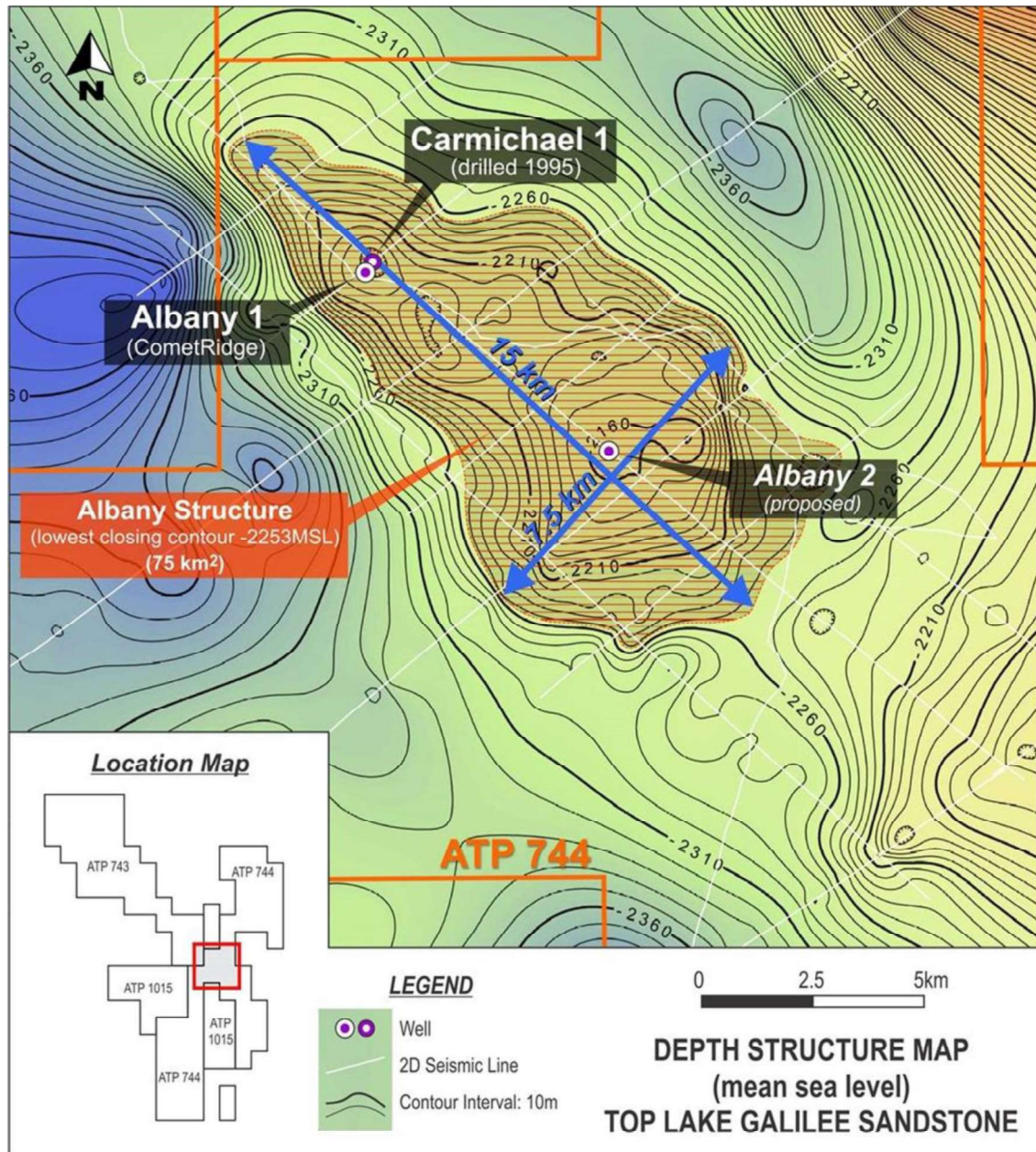
Figure 30. Revised mapped extent of Albany structure
