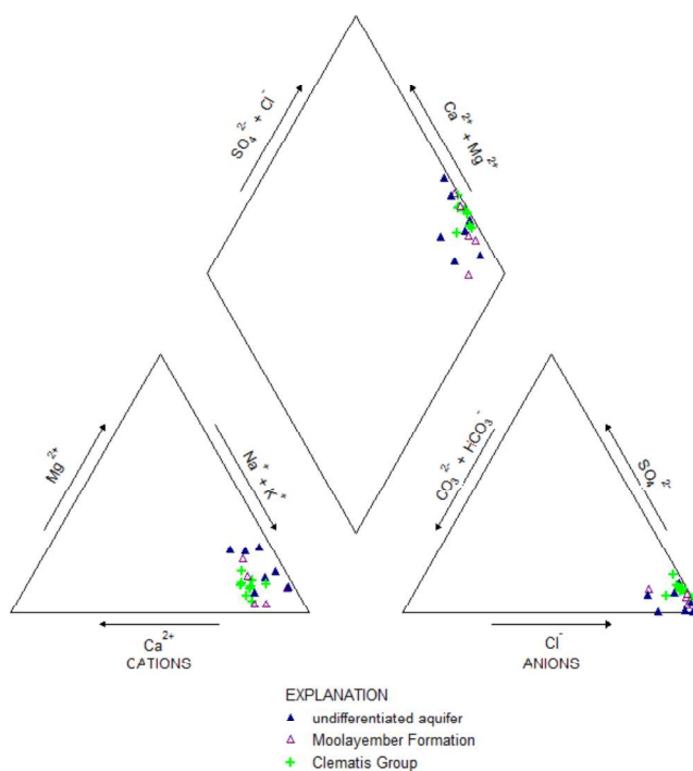
Figure 19: Piper Diagram for all available quality data within ATP 744 (excluding analysis from Gunn #2 and DST's)
