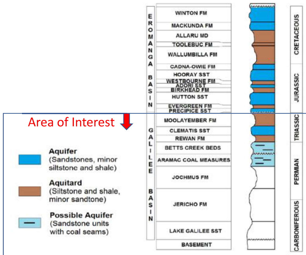
Figure 35. Simplified hydrostratigraphy in the Galilee and Eromanga Basins (after Mooya, 2011)
