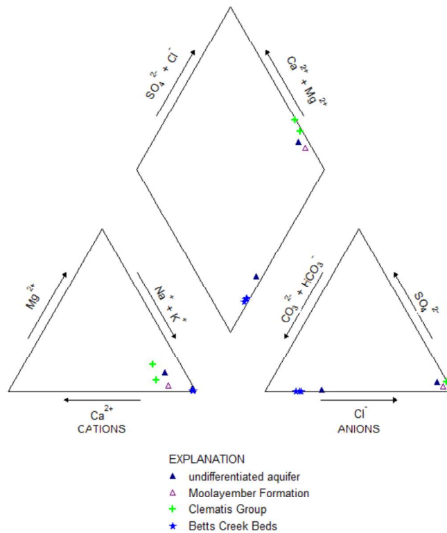
Figure 20: Piper Diagram for all available quality data from Betts Creek Beds at Gunn #2 and within 20km of Gunn #2 (excluding analysis from DST's)
