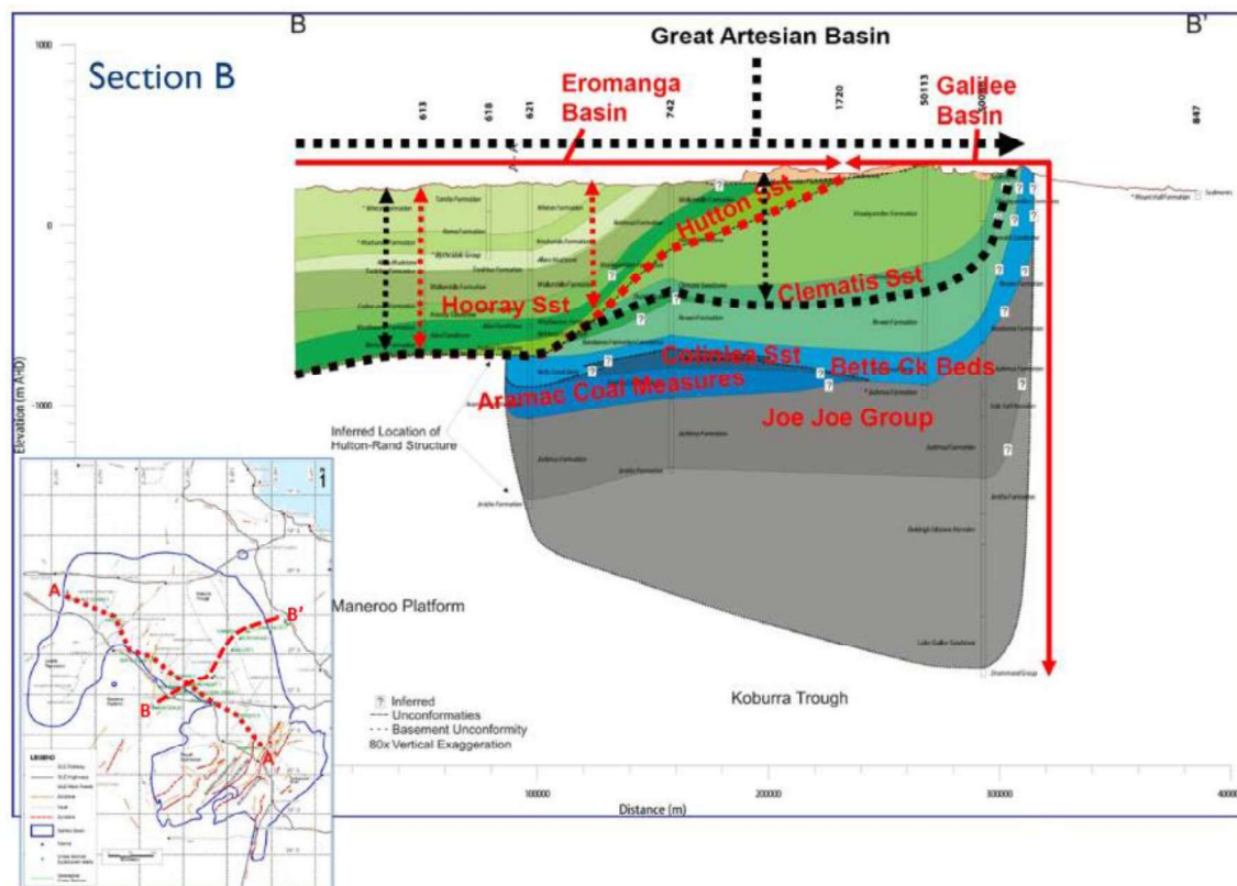
Figure 34. East to west stratigraphic cross section of the Galilee Basin (RPS 2012).
